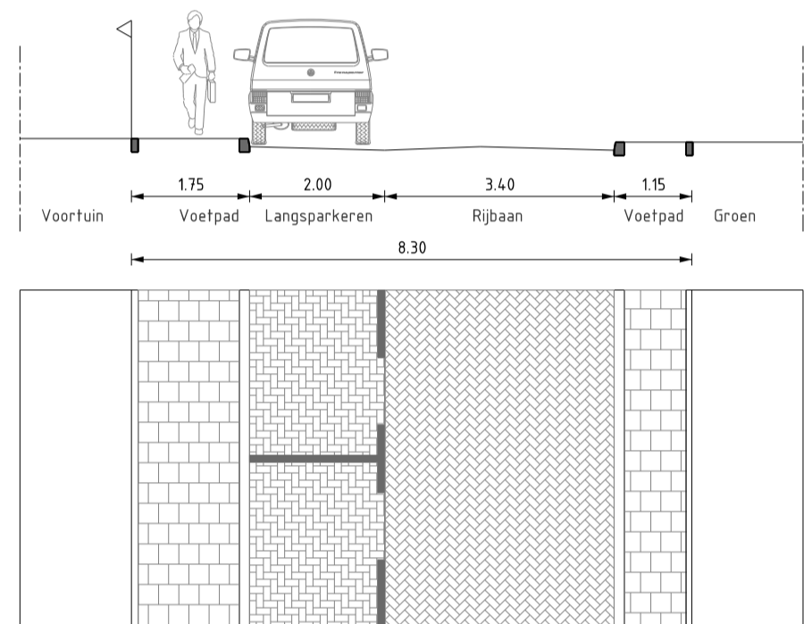
PROFIEL 53 SCHAAL 1 : 100 VO-03 Insulindesingel (west)
