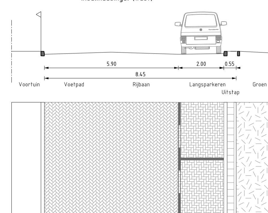
PROFIEL 62 SCHAAL 1 : 100 VO-03 Insulindesingel (west)
