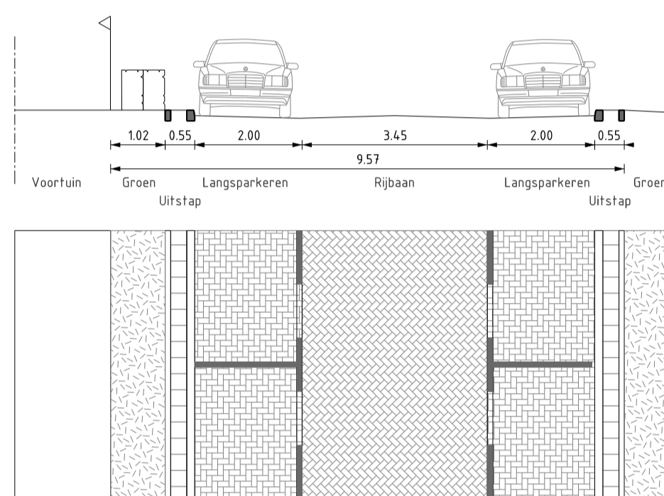
PROFIEL 51 SCHAAL 1 : 100 VO-03 Insulindesingel (west)
