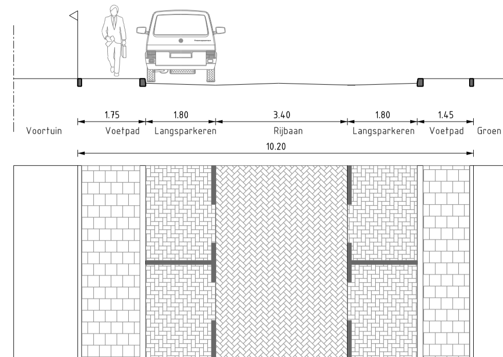
PROFIEL 48 SCHAAL 1 : 100 VO-03 Insulindesingel (west)
